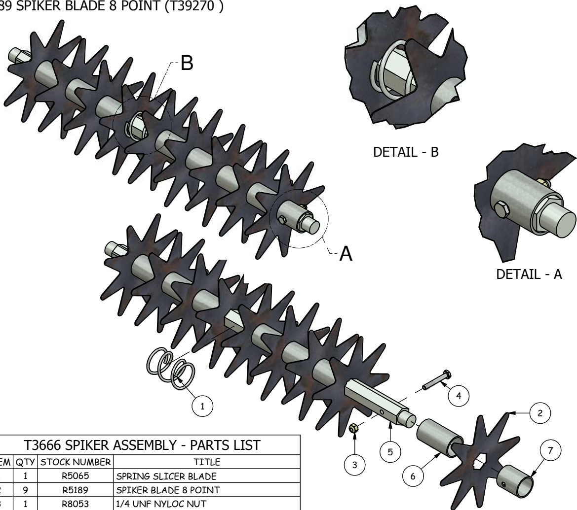
R5189 SPIKER BLADE 8 POINT (T39270 )
