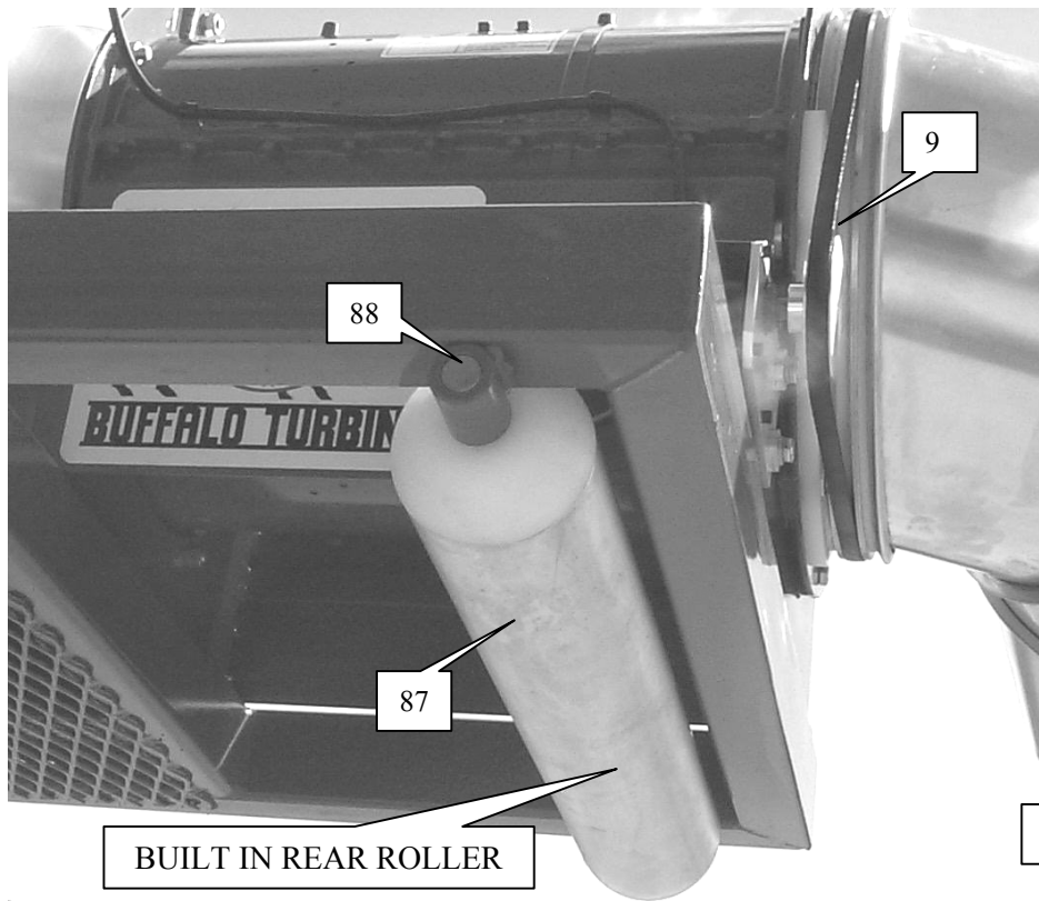
Bottom View of Hurricane/PTO
